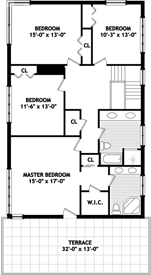
2nd FLOOR
