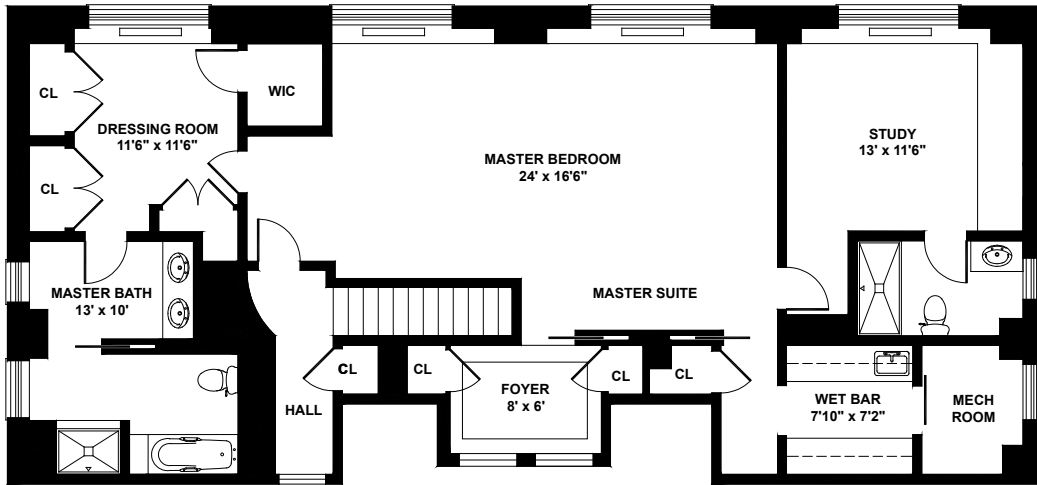
UPPER LEVEL
