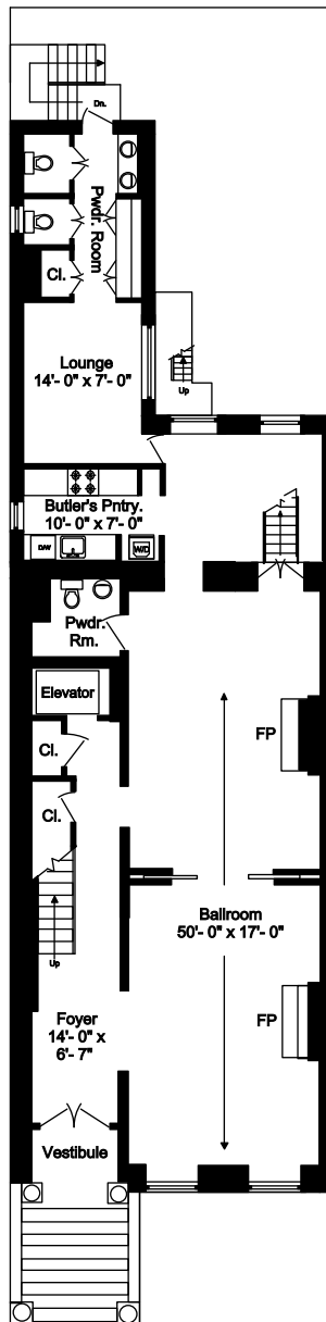
Parlor Floor
