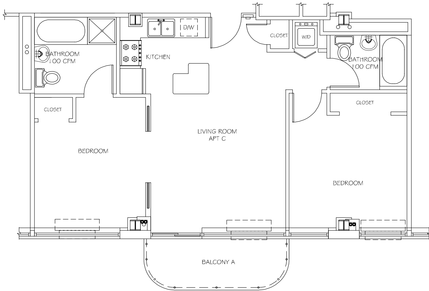
TYPICAL (3RD - 12TH) APT C FLOOR AREA: 796.2 SQFT BALCONY A: 65.6 SQFT
