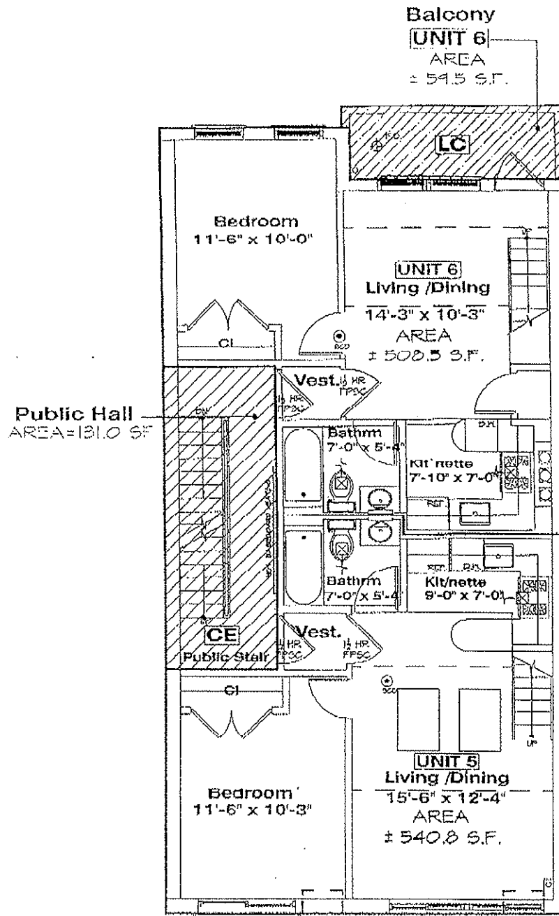
PROPOSED FOURTH FLOOR PLAN N.T.S.
