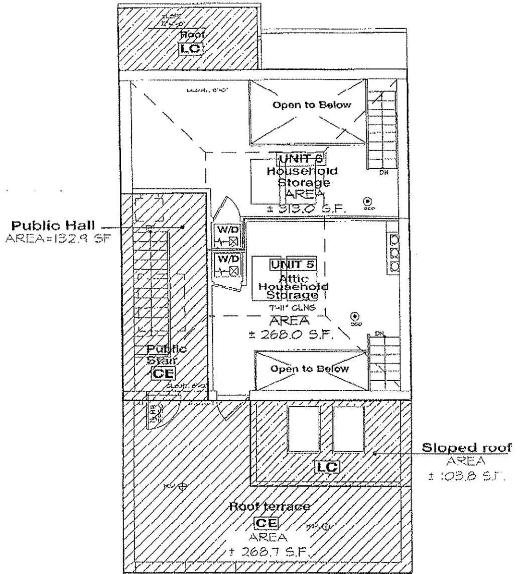
PROPOSED ATTIC PLAN N.T.S.
